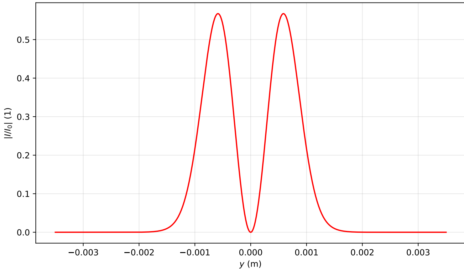
Intensity profile I(x=0, y, z=1.194)/I_0 , P_{in}=0.5P_{cr} , artificial time
